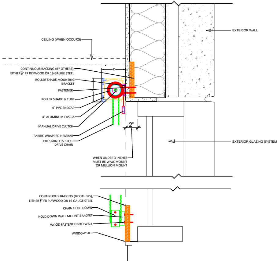
3 SINGLE MANUAL ROLLER SHADE WALL MOUNT/ TYPICAL NOT TO SCALE
