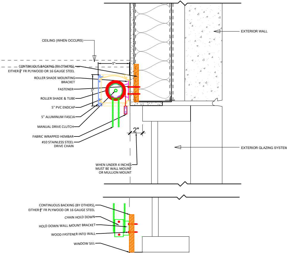
3 SINGLE MANUAL ROLLER SHADE WALL MOUNT/ TYPICAL NOT TO SCALE
