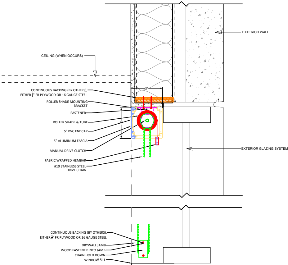
2 SINGLE MANUAL ROLLER SHADE TOP MOUNT/ TYPICAL NOT TO SCALE
