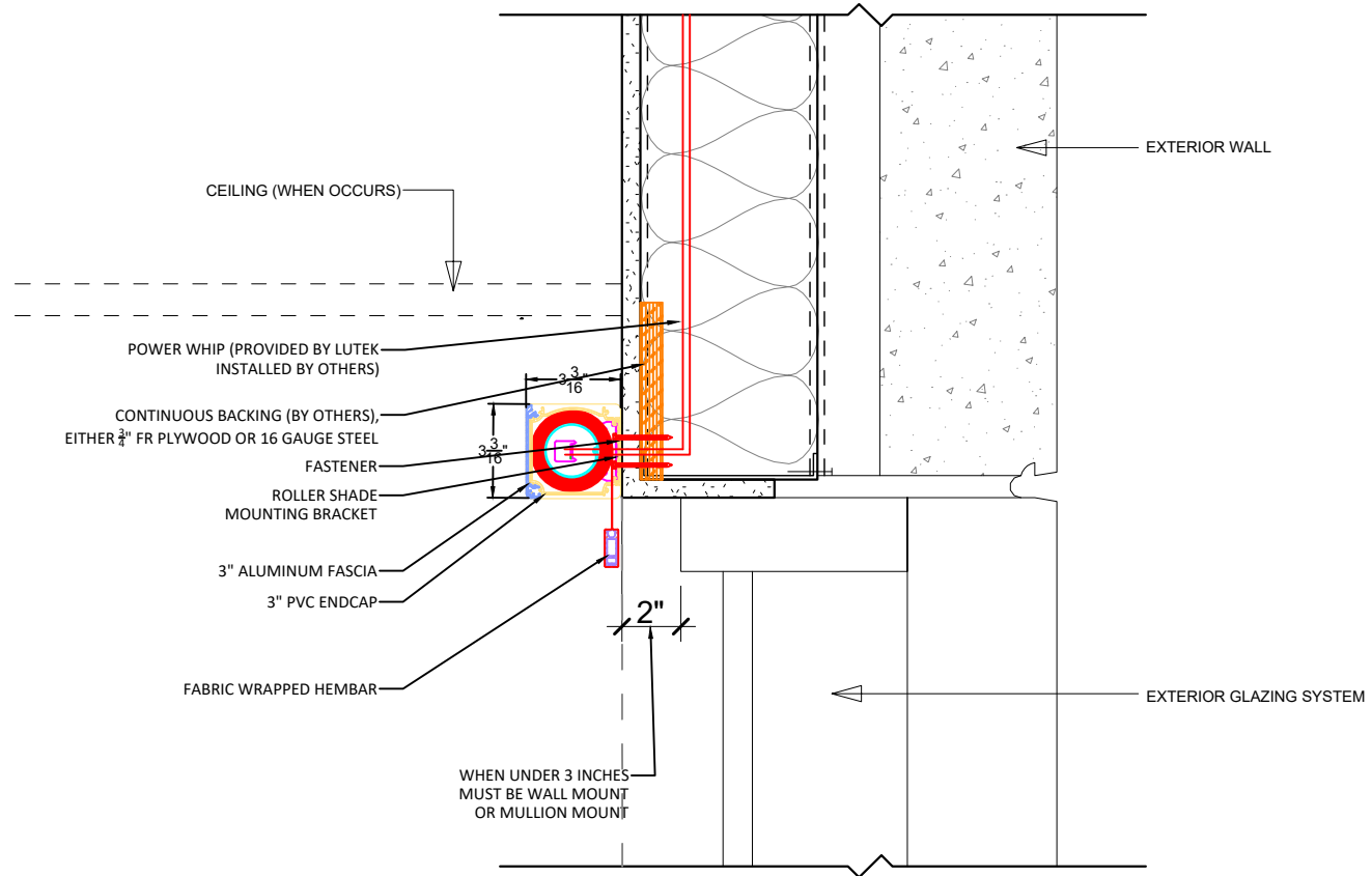
3 SINGLE MOTORIZED ROLLER SHADE WALL MOUNT/ TYPICAL NOT TO SCALE
