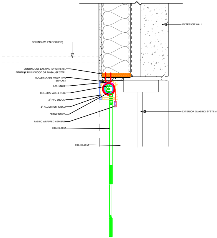
2 SINGLE CRANK ROLLER SHADE TOP MOUNT/ TYPICAL NOT TO SCALE
