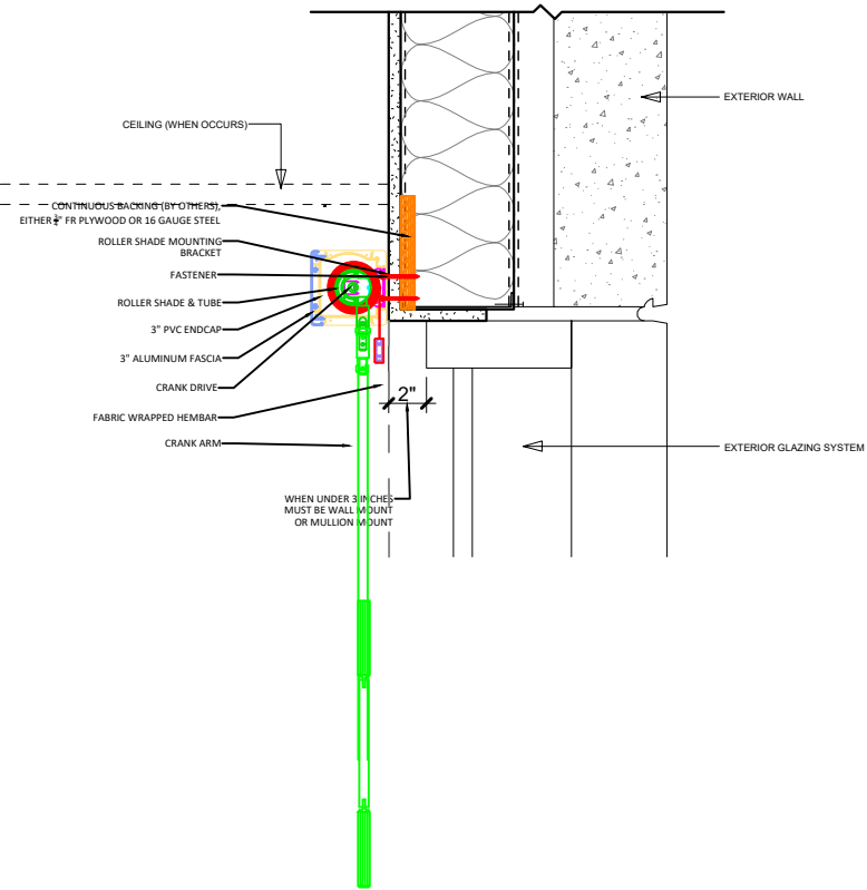
3 SINGLE CRANK ROLLER SHADE WALL MOUNT/ TYPICAL NOT TO SCALE
