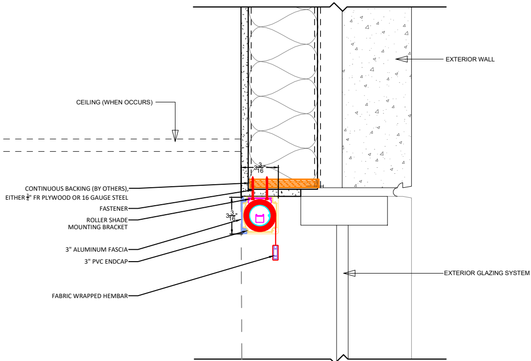
2 SINGLE CORDLESS ROLLER SHADE TOP MOUNT/ TYPICAL NOT TO SCALE
