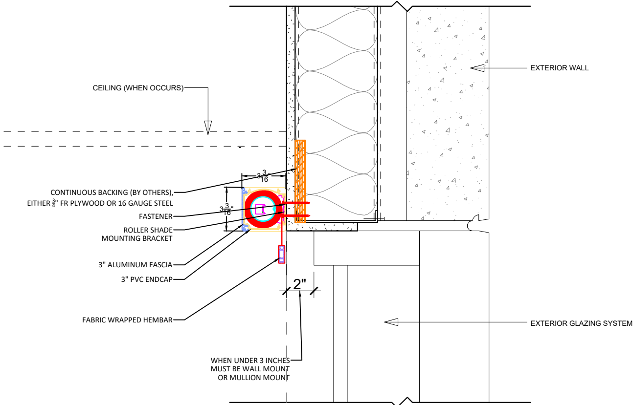
3 SINGLE CORDLESS ROLLER SHADE WALL MOUNT/ TYPICAL NOT TO SCALE
