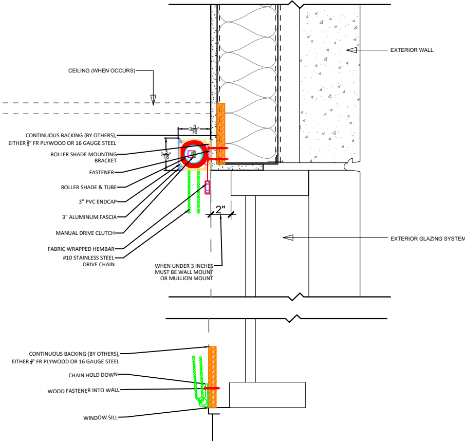
3 CONTRACT SUITE ROLLER SHADE WALL MOUNT/ TYPICAL NOT TO SCALE
