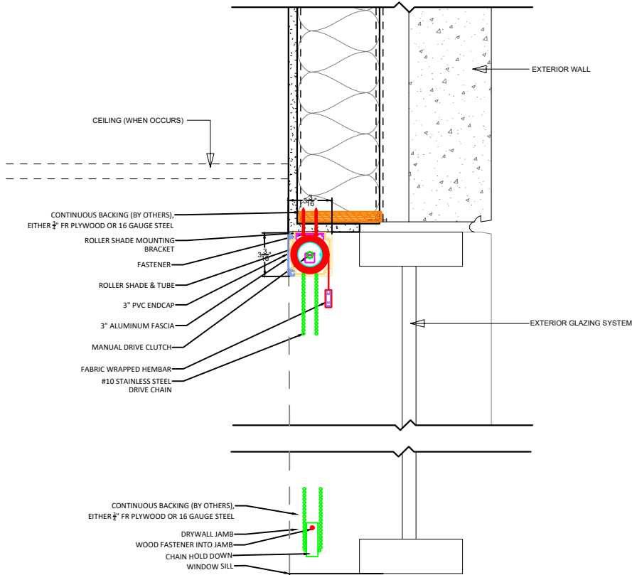
2 CONTRACT SUITE ROLLER SHADE TOP MOUNT/ TYPICAL NOT TO SCALE
